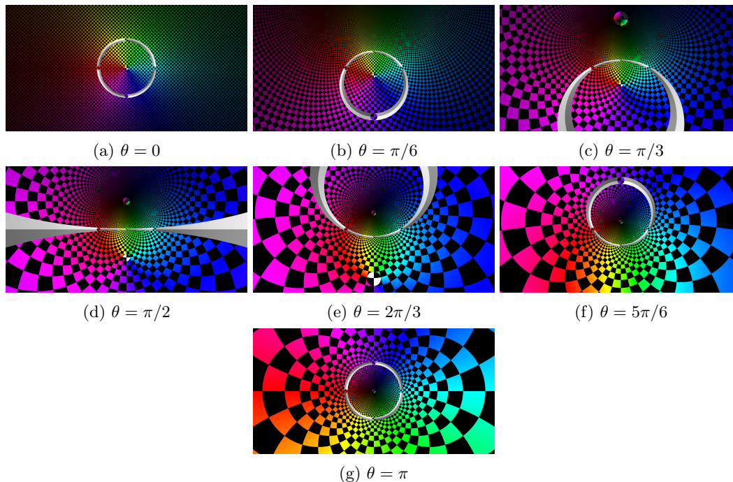
FIG. 2: Visualisations of \mathcal{R}_x(\zeta; \theta) over the course of a half rotation of the Riemann sphere about the x -axis. Initially the eye is at the South Pole looking up, so the North Pole ( \zeta = 0 , white/black circle) is directly overhead. After rotating by \theta = \pi/2 , the point \zeta = i on the equator (green circle and grey unit disc respectively) is overhead. After rotating to \theta = \pi , the South Pole ( \zeta = \infty , black ring with multicoloured interior) is overhead. See https://github.com/RCPN/Spinors for interactive versions that you can play with at home. (Plots made using David Bau's Conformal Map Viewer http://davidbau.com/conformal/#z .)
